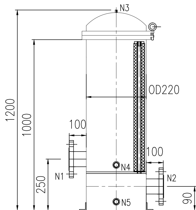
NOZZLE ORIENTATION
